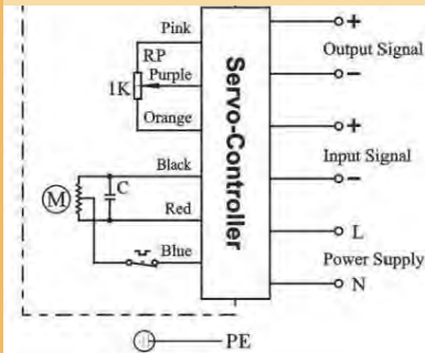
Type E: With Servo Controller (Adjusting Type)
