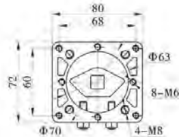
Explosion Proof Standard Type
