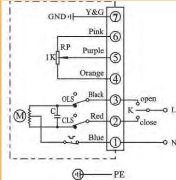
Type C: with 1K \Omega (or 500 \Omega ) Potentiometer
